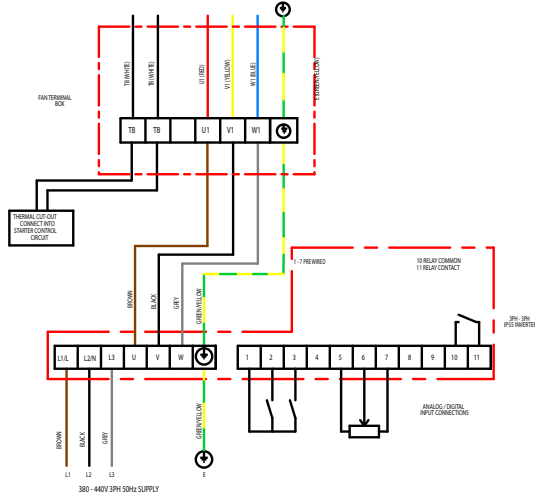
VARIABLE SPEED CONNECTION CONTROLLER TYPE 3PH - 3PH IP55 INVERTER
